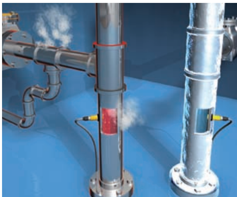
Can stand the heat: When things start to heat up, certain capacitive Turck sensors can withstand temperatures of 100 °C
